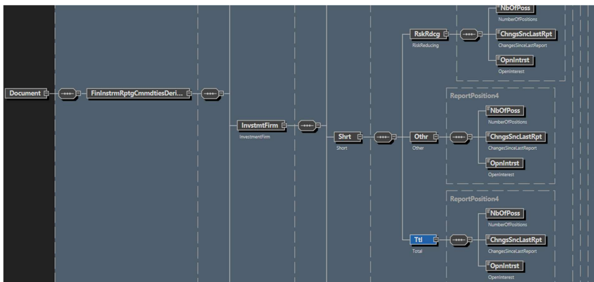
FIGURE 3 - XSD SCHEMA STRUCTURE – LONG/ SHORT POSITION
